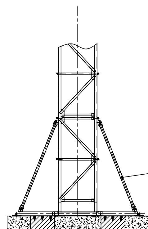
A向 (省略吊笼) (View A, omitting cage)
